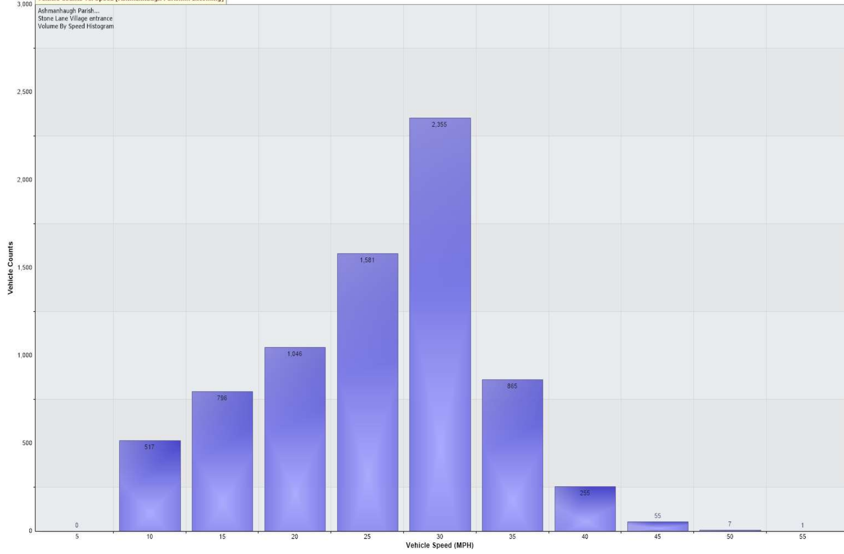
Vehicle Counts Vs. Speed [Ashmanhaugh Parish...: Incoming]
