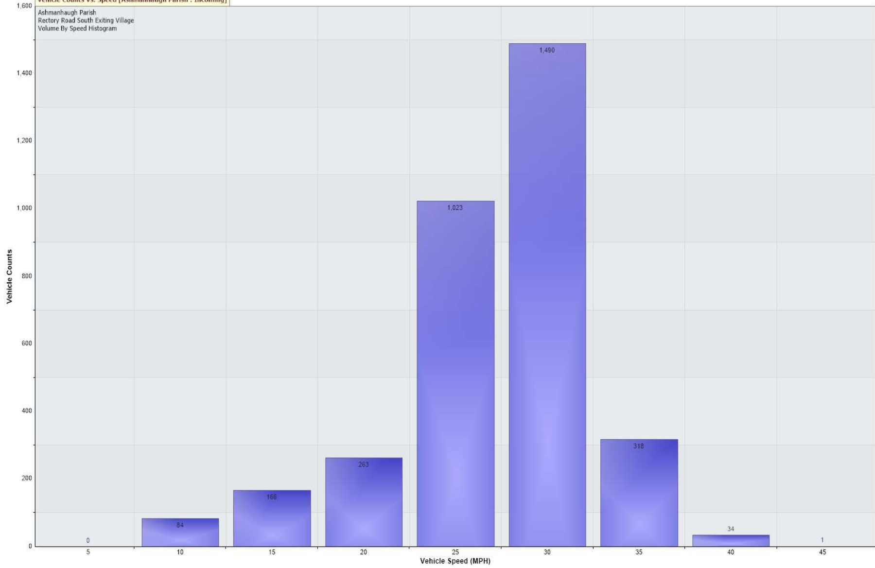
Vehicle Counts Vs. Speed [Ashmanhaugh Parish : Incoming]
