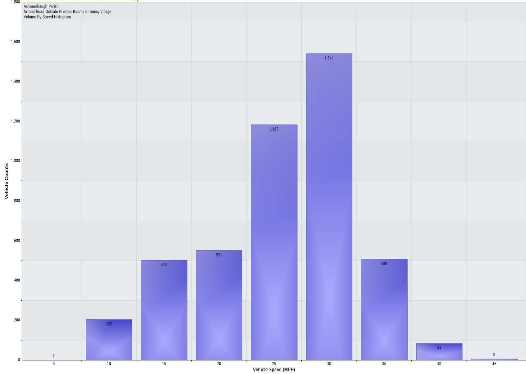
Vehicle Counts Vs. Speed [Ashmanhaugh Parish: Incoming]
